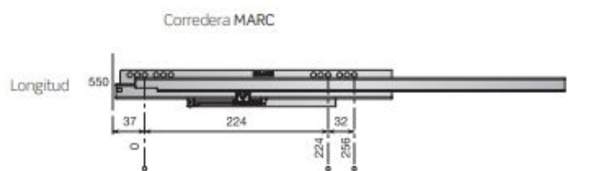
Enganche frontal
